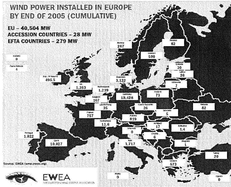
Figure 1.11: Installed Wind Power Capacities in Europe
