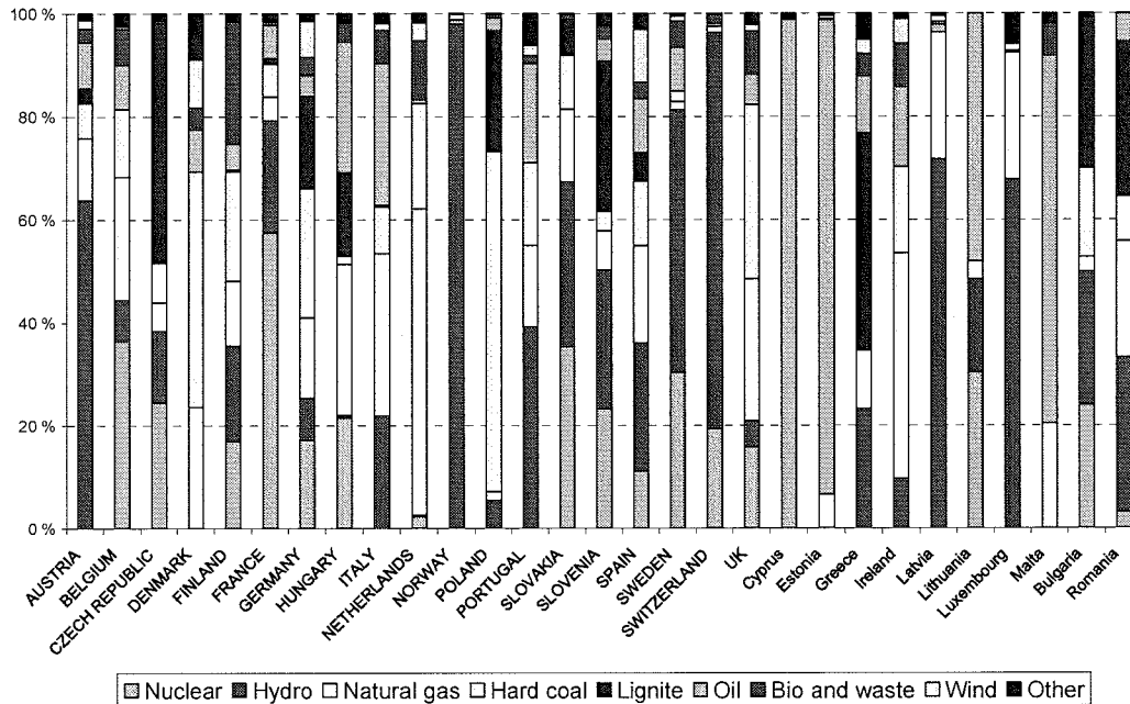
Figure 1.9: Composition of electricity generation capacity in Europe
